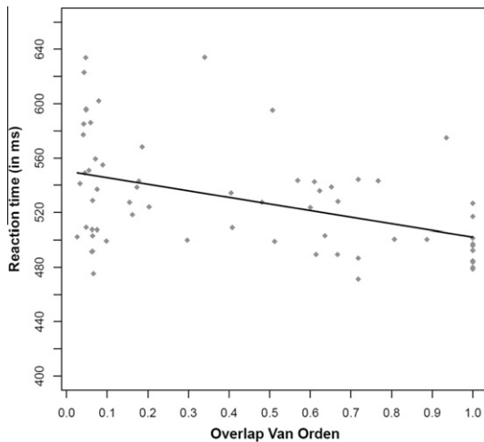
Fig. 1. Graph depicting the decrease in RT as a function of cross-lingual overlap on mean target RTs in Experiment 1. The straight line represents the best linear fit.
