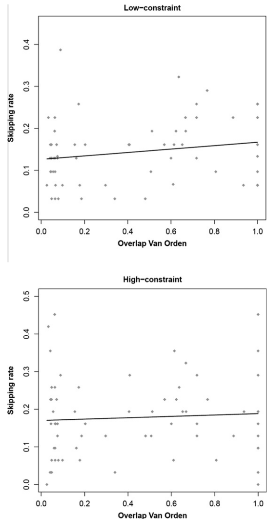
Fig. 3. Graph depicting the increase in skipping rate as a function of cross-lingual overlap on mean target skipping rates in low- and high-constraint sentences in Experiment 2. The straight line represents the best linear fit.
