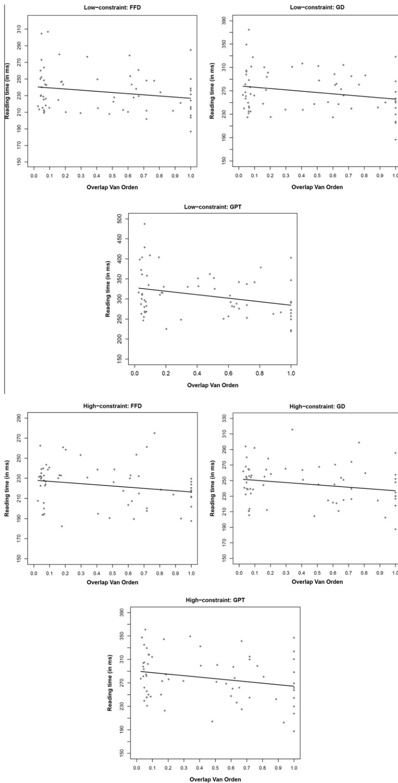
Fig. 2. Graphs depicting the decrease in First fixation duration (FFD), Gaze duration (GD), Go-past time (GPT) as a function of cross-lingual overlap on mean target reading times in low- and high-constraint sentences in Experiment 2. The straight line represents the best linear fit.
