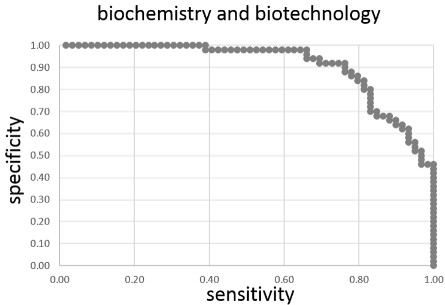
Figure 1. ROC Curve for the Program biochemistry and biotechnology .
