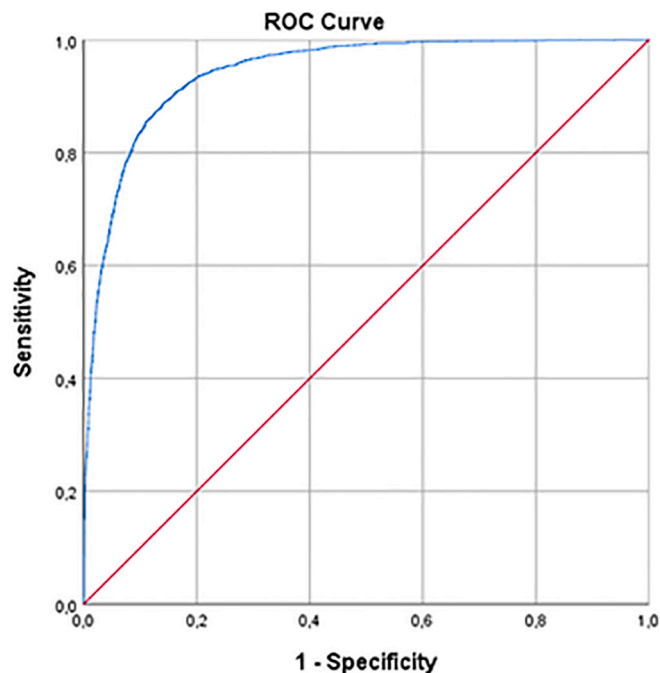
Fig. 2. The ROC Curve of STEM Study Choice versus non-STEM Study Choice.
