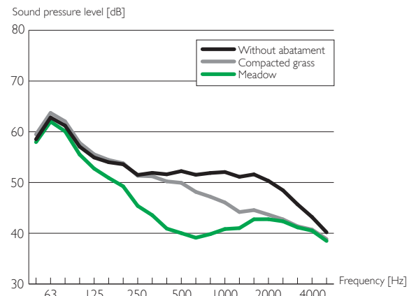
Two types of grass-covered ground. Sound-pressure-level spectra predicted for a 1.5-m-high receiver located 50 m from the nearest traffic lane (5% heavy and 95% light vehicles, travelling at 50 km/h) for compacted grass (grey), meadow (green) and hard ground (black) between road edge and receiver. Predicted insertion loss: 5 dB(A) for compacted grass and 8 dB(A) for meadow.
