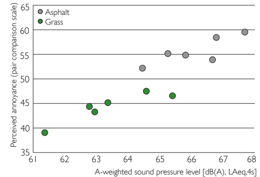
Recordings along a tramway line bordered by hard (left) and soft ground (middle). The diagram shows the results of a listening experiment in which 29 listeners assessed the perceived annoyance of tram passages recorded at a point 7 m from the track, bordered by soft (green) or hard (grey) ground.
