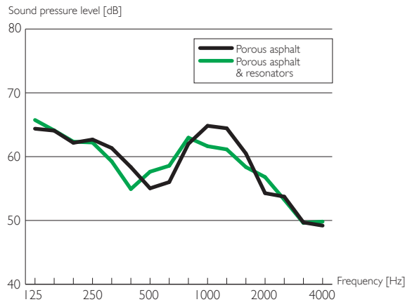
Sound-pressure-level spectra (left) and maximum A-weighted sound pressure levels (below) from pass-by measurements over porous asphalt with and without buried resonators (light vehicle rolling noise at 100 km/h, for a 1.2-m-high receiver located 7.5 m from the road). The addition of resonators increases the insertion loss with approximately 3 dB(A).
