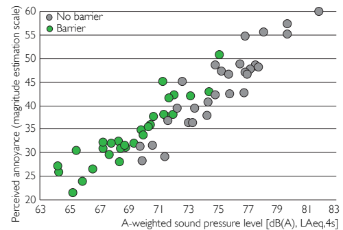
Recordings made using “artificial head technology” to obtain high-quality recordings for listening experiments. Diagram: Results of a listening experiment in which 31 listeners assessed the perceived annoyance of traffic noise events recorded at barrier-shielded (green) or non-barrier-shielded (grey) places along the road.
