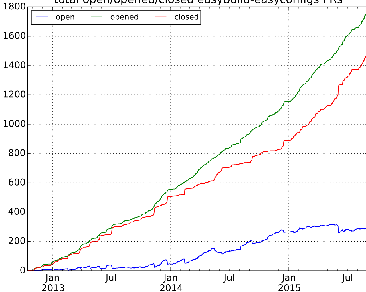
total open/opened/closed easybuild-easyconfigs PRs
