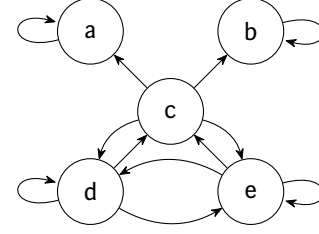
Figure 1. \bar{\mathcal{G}}(\bar{T}) for Running example 1.
