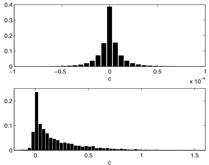
Fig. 5. The histogram of the values of the pairwise redundancy c_{ij} , in fMRI example (bottom), and choosing randomly the modes u (top).
