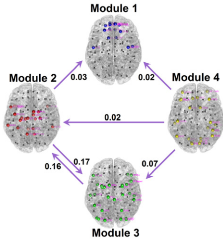
Fig. 6. The causalities between the four modules of the fMRI application.
