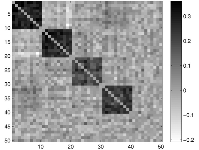
Fig. 1. The correlation matrix of the simulated example, showing four groups of variables correlated at equal times.
