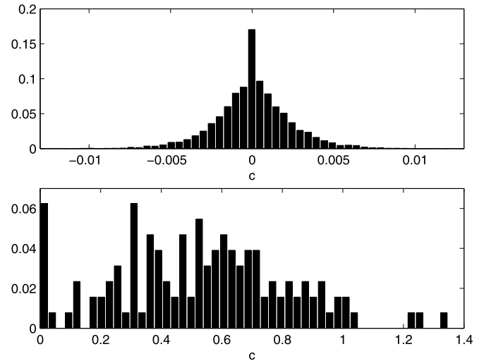
Fig. 8. The histogram of the values of the pairwise redundancy c_{ij} , in genetic application (bottom), and choosing randomly the modes u (top).
