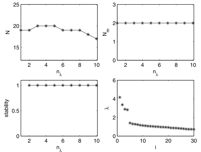
Fig. 2. (Top-left) Concerning the simulated example, the number of selected variables N is plotted versus n_\lambda , the number of modes. (Top-right) The number of modules, obtained by modularity maximization, of the matrix c_{ij} , whose elements measure the pairwise redundancy. (Bottom-left) The measure of the stability of the partition, going from n_\lambda - 1 to n_\lambda , is plotted versus n_\lambda . (Bottom-right) The eigenvalues of the matrix x^T x are depicted.
