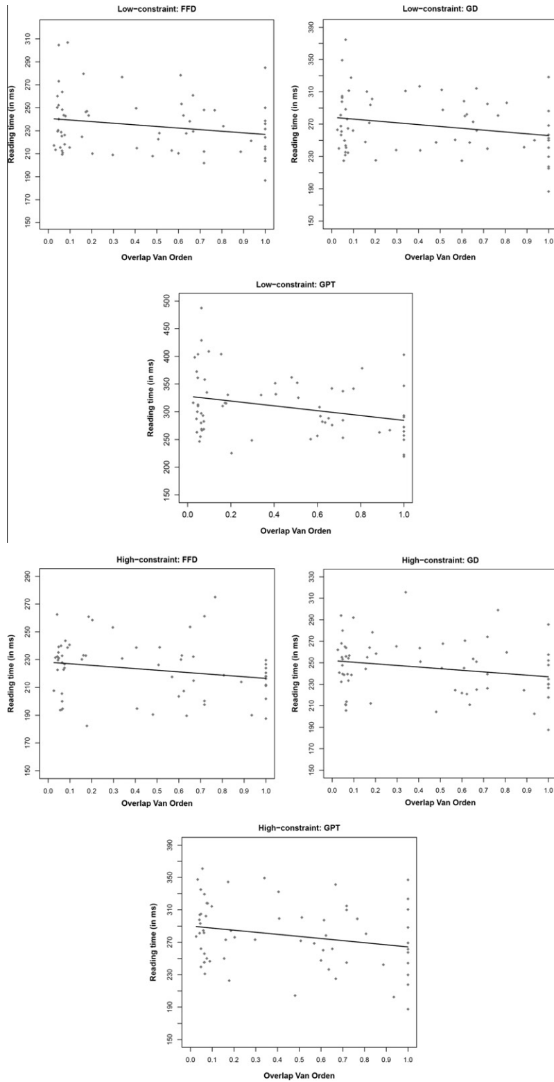
Fig. 2. Graphs depicting the decrease in First fixation duration (FFD), Gaze duration (GD), Go-past time (GPT) as a function of cross-lingual overlap on mean target reading times in low- and high-constraint sentences in Experiment 2. The straight line represents the best linear fit.
