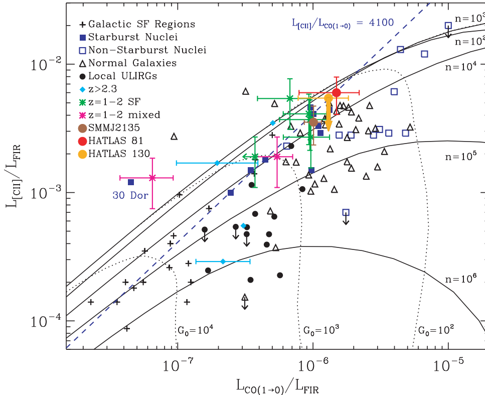
Figure 4. Diagnostic diagram of L_{[\text{C II}]} / L_{\text{FIR}} as a function of L_{\text{CO}(1-0)} / L_{\text{FIR}} for SDP.81 (the rightmost filled circle) and SDP.130 (filled circle with a down arrow), compared to local and other known high-redshift galaxies of different classes (Stacey et al. 1991, 2010; Hailey-Dunsheath et al. 2010). The lines with the constant density n and constant G_0 from PDR models of Kaufman et al. (1999) are also shown. The [C II] luminosity was corrected for the fraction of the flux arising from H II and diffuse ionized regions. The CO(1–0) line flux from the EVLA measurement was multiplied by 2 to take into account that the line is optically thick and we see only the fraction coming from the illuminated PDR side. L_{[\text{C II}]} / L_{\text{CO}(1-0)} of 4100, typical for local starburst galaxies, is also shown as a dashed line. We have used L_{\text{FIR}}(42.5\text{--}122.5\ \mu\text{m}) = L_{\text{IR}}(3\text{--}2000\ \mu\text{m}) / 1.54 , derived by integrating the SED of SDP.81.
