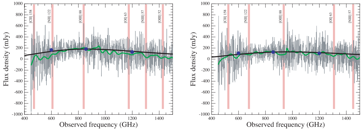
Figure 2. The FTS high- and low-resolution spectra of SDP.81 (left-hand panel) and SDP.130 (right-hand panel) overlaid with the three SPIRE photometric points (dots) and the SED template fit. The photometric errors, even including the 7 per cent flux calibration uncertainty of the SPIRE Photometer, are smaller than the dots. The expected positions of a number of fine-structure lines are indicated with vertical bars.
