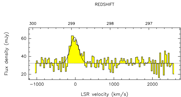
Fig. 1. Spectrum of the para H 2 O 2 02 –1 11 emission line towards SDP.17b, where the velocity scale is centred on its observed frequency at 298.93 GHz (corresponding to z = 2.3049 ). The rms noise is \sim 4.7 mJy/beam in 31.6 MHz channels. A Gaussian fit to the H 2 O spectrum is shown as a solid line while the dotted line shows the underlying dust continuum emission. The H 2 O line is clearly asymmetric and not well fit by a Gaussian profile.
