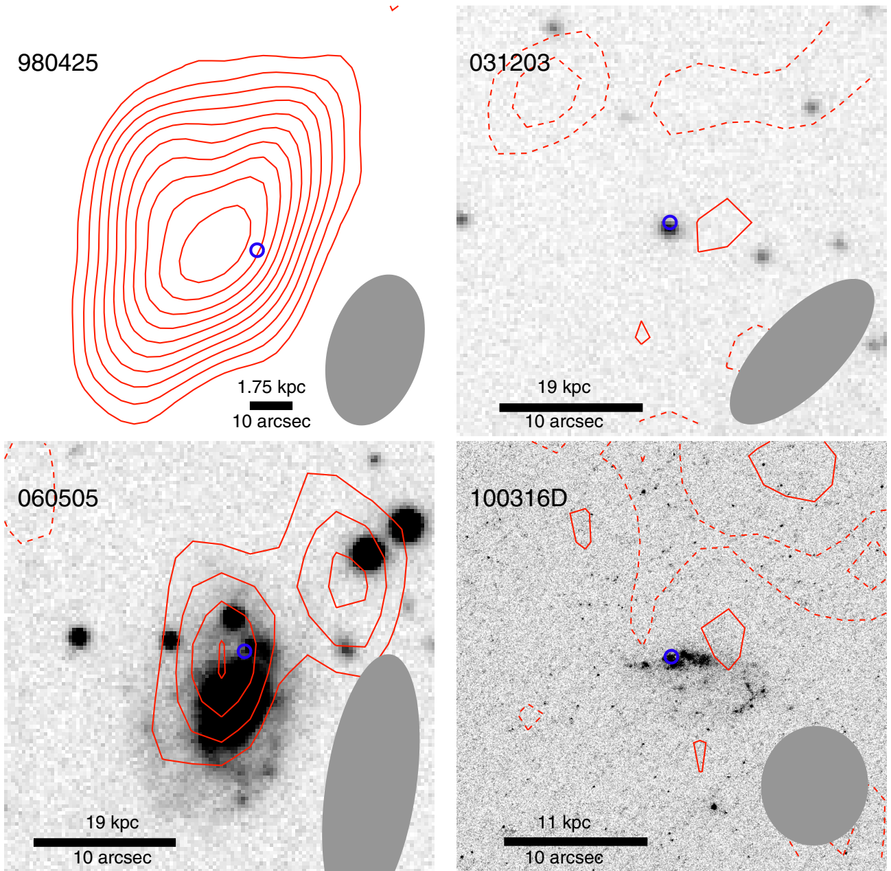
Fig. 1. Integrated HI line map of the GRB hosts (contours; positive/negative values are solid/dashed at -2, -1, 2, 3, 4\sigma, \dots ) on top of the optical images (Sollerman et al. 2005; Mazzali et al. 2006; Thöne et al. 2008; Starling et al. 2011). The spectrum was integrated in the frequency range shown as dotted lines in Fig. 2. North is up and east is to the left. The images are 30'' \times 30'' except for GRB 980425, for which it is 100'' \times 100'' . The scale is indicated on each panel. The FWHM beam sizes of the HI data are shown as filled ellipses. The blue circles show the GRB positions. The map for the GRB 111005A host is not shown, as we use archival data with poor spatial resolution (Sect. 2.1). To estimate the HI properties for the GRB 060505 host only the central source was used. The north-western source is at the same redshift (Fig. 2) and is analysed separately (Table 4 and Sect. 4.3).
