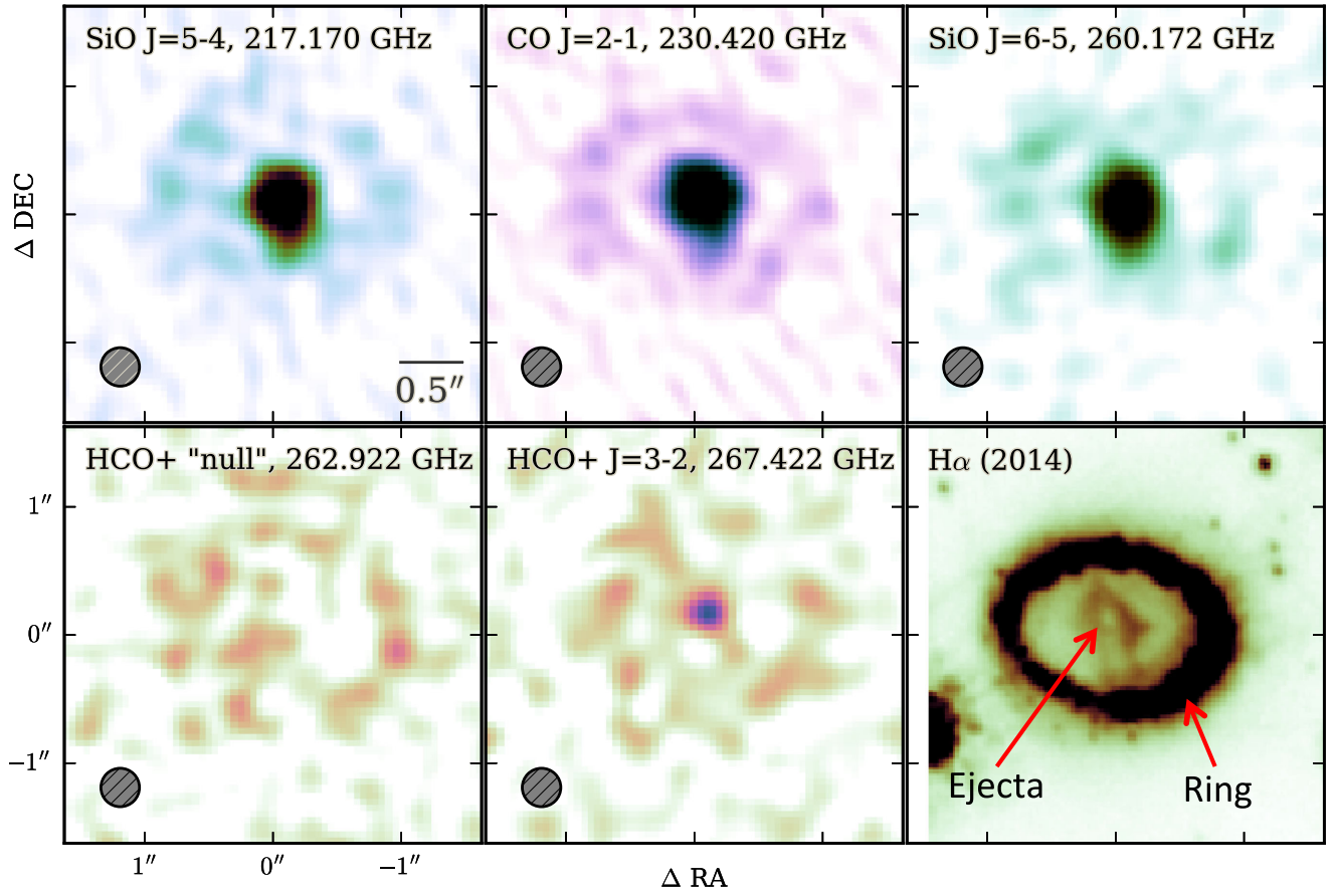
Figure 1. The ALMA 217, 230 and 267 GHz images, along with a Hubble Space Telescope H \alpha image (Fransson et al. 2015; Larsson et al. 2016). The SiO and CO lines originate from the ejecta, located in the centre of the ring. The faint emission from the ring seen in all ALMA images, is due to synchrotron radiation from the ring. The quoted frequencies are those observed, rather than the line centre. The HCO ^+ 267.4 GHz line is clearly detected in the ejecta, when comparing with the ‘null’ frequency image at 262.9 GHz.
