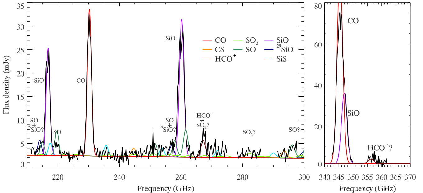
Figure 2. The ALMA 210–300 and 340–360 GHz spectra of SN 1987A’s ejecta (black). Major molecular features are labelled. Model molecular spectra with a 2000 km s ^{-1} FWHM Gaussian line profile and the excitation temperature of 40 K, are plotted in colour, guiding molecular identifications. Underlying synchrotron radiation, leaked from the ring into the aperture, is represented by a power law with an index of -0.8 .
