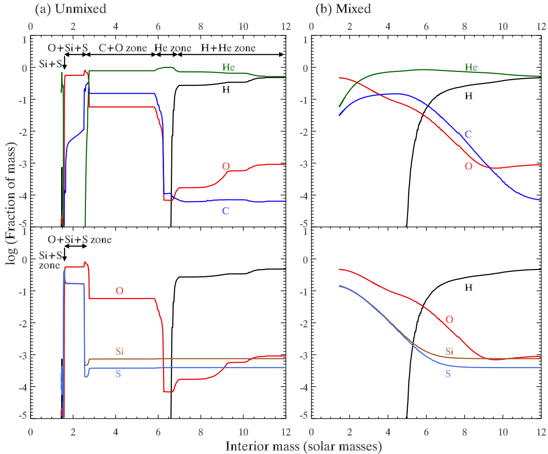
Figure 10. The modelled fractional abundance of atoms after SN explosion. The x -axis shows the interior stellar mass, with zero M_{\odot} being the inner most. The model is an 18 M_{\odot} star with one-third of the solar metallicity based on the model for Sk-69° 9202 (Sukhbold et al. 2016), but involving more extensive nuclear reaction network. Only the inner 12 solar masses of the 17.09 M_{\odot} solar mass pre SN are shown. Panel (a) shows SN 1987A model without mixing of nuclear-burning zones. Panel (b) shows an example of the effect of mixing, with the model with artificial mixing at t = 10^7 s. For clarity, we split the plots in two (upper and lower panels). The upper panel is for ^1\text{H} , ^4\text{He} , ^{16}\text{O} and ^{12}\text{C} , and the lower panel is for ^{28}\text{Si} and ^{32}\text{S} with H and O for guidance. The unmixed model (a) shows distinct nuclear-burning zones, Si+S, O+Si+S and C+O zones, as well as He and H+He envelopes. (b) Having mixing triggered by the explosion can make elements from different nuclear-burning zones mixed to some degree, though the degree of mixing is largely in debate. The most notable effect of mixing is Si and S being mixed into O (right lower panel), which was not the case in the unmixed model (left lower panel).
