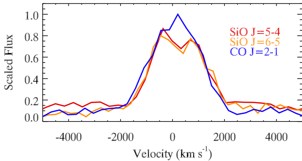
Figure 3. The line profiles of SiO J = 5-4 and 6-5 , compared with that of CO J = 2-1 . The SiO lines clearly show dips at the top at \sim 300 km s^{-1} . An LMC systemic velocity of 275 km s^{-1} has been subtracted from all spectra.
