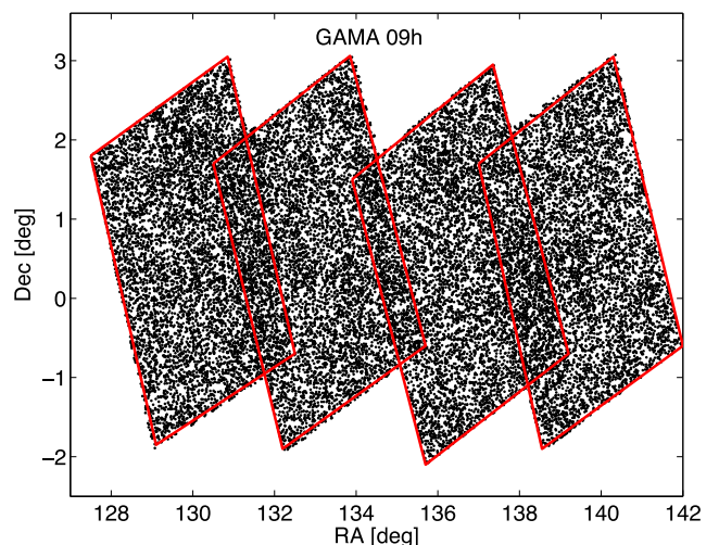
Figure 1. Distribution of selected H-ATLAS sources in the 9 h equatorial field (one-third of the total equatorial regions). The field is made of four partially overlapping areas, referred to as ‘tiles’.
