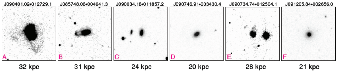
Figure 7. SDSS postage stamp images in the r band ( 70 \times 70 \text{ arcsec}^2 ) of galaxies corresponding to the marked data points in Fig. 6. Images are sorted (left-to-right) according to the estimated dust temperature. The SDSS optical major isophotal diameter in the r -band (e.g. isoA-r ) has been used to measure the optical linear diameter of each galaxy D_{25} in units of kpc as indicated on each panel.
