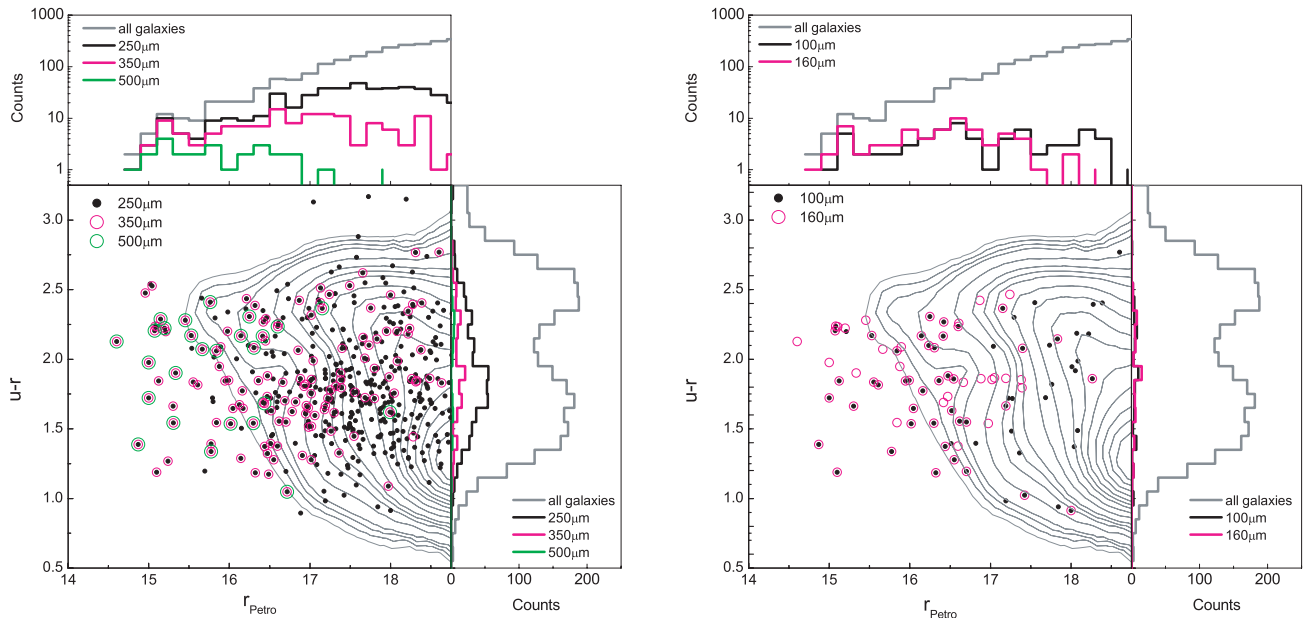
Figure 1. Colour–magnitude diagram of optically selected galaxies (grey contour lines) and their submillimetre counterparts with \text{Reliability} \geq 0.8 detected at \gtrsim 5\sigma by SPIRE (left-hand panel) and PACS (right-hand panel). Horizontal and vertical histograms show the distribution of galaxy optical colour ( u - r ) and r -band magnitude ( r_{\text{Petro}} ), respectively. Colours represent: ‘grey’ all galaxies; ‘black’ sources with SPIRE 250 \mu\text{m} (left-hand panel) and PACS 100 \mu\text{m} (right-hand panel) detections; ‘pink’ sources with SPIRE 350 \mu\text{m} (left-hand panel) and PACS 160 \mu\text{m} (right-hand panel) detections; ‘green’ sources with SPIRE 500 \mu\text{m} detections.
