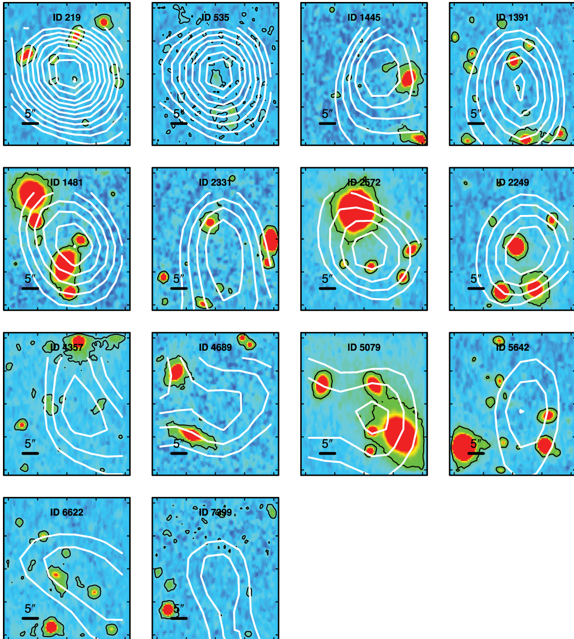
Figure 5. Co-added 40 \times 40 \text{ arcsec}^2 gri images of the 14 strong lens candidate H-ATLAS sources for further study and follow-up (centred on the 250 \mu\text{m} positions, with 250 \mu\text{m} contours starting at 3\sigma and increasing in steps of 1\sigma ) within 1 arcmin ( \simeq 0.2 \text{ Mpc} ) of the cluster centres in order of decreasing 250 \mu\text{m} flux density (left–right, top–bottom).
