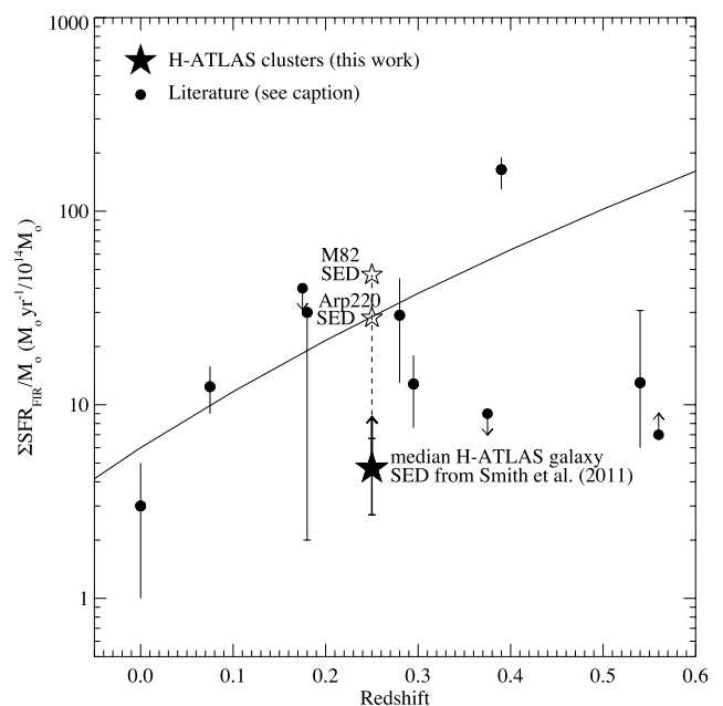
Figure 4. Measures of the mass-normalized SFRs in galaxy clusters out to z \sim 0.6 , adapted from fig. 6 of Geach et al. (2006). The SFRs are derived from the mid- or far-infrared populations within \sim 2 Mpc and are normalized to the best estimate of the total (luminous+dark) cluster mass. Listed in order of increasing redshift, they are Perseus (Meusinger, Brunzendorf & Krieg 2000), A3112 (Braglia et al. 2011), A2218 (Biviano et al. 2004), A1689 (Fadda et al. 2000; Duc et al. 2002), H-ATLAS (this work), A1758 (Haines et al. 2009), the Bullet cluster (Clowe, Gonzalez & Markevitch 2004; Markevitch 2006; Rawle et al. 2010), A370 (Metcalf, Fadda & Biviano 2005), Cl0024+16 and MS0451–03 (Geach et al. 2006) and J1888.16LC (Duc et al. 2004). An evolutionary model for the counts of star-forming ULIRGs from Cowie et al. (2004) is overlaid as a guide only, and has been normalized arbitrarily to the mean SFR in Cl0024+16 and MS0451–03 from Geach et al. (2006). This plot shows an increasing rate of activity in more distant clusters as traced through their mid- or far-infrared populations, albeit with a large scatter, suggestive that the infrared is a sensitive tracer of environmental changes within the clusters. Note that there are large systematic effects on the points in this plot, with the inferred SFR dependent on the assumed form of the SED, and estimate of the total cluster mass. Given the large uncertainties on the H-ATLAS cluster masses and the cool SED we have adopted, we consider our point a lower limit (as indicated by the arrow). We also show how our result changes if we instead assume an M82 or Arp220 SED (open symbols), to facilitate a comparison with the literature results.
