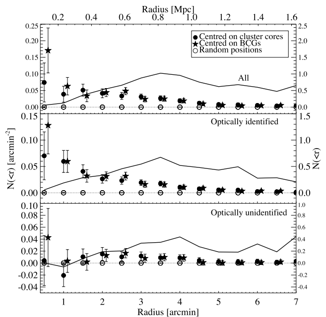
Figure 2. Cumulative number density of the average background-subtracted (points; axis on the LHS) and number (curve; axis on the RHS) of all (top panel), optically identified (middle panel) and optically unidentified (bottom panel) H-ATLAS sources as a function of clustocentric radius. For comparison, we have also plotted the average (background-subtracted) cumulative surface density as a function of radius from the central BCG (stars). The standard error of the mean has been used to calculate the error bars. This plot shows that we have measured an excess of H-ATLAS sources (with the significance varying with radius) within a projected clustocentric radius of 5 arcmin (which corresponds to 1.2 Mpc at z = 0.25 ) over that of the background field H-ATLAS sources, with optically identified sources (presumably far-infrared-bright cluster members, see text) making the most significant contribution to the measured excess. For reference, the average area of a single cluster is 7.5 \text{ arcmin}^2 , where the area is defined to contain 80 per cent of the cluster members originally assigned by the Voronoi tessellation detection.
