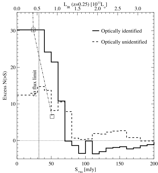
Figure 3. Background-subtracted cumulative number counts of optically identified and unidentified H-ATLAS sources within 5 arcmin of the 66 cluster cores. The 250\ \mu\text{m} 5\sigma flux limit of the H-ATLAS catalogue is shown by the dotted vertical line. Based on the far-infrared colours, we expect most of the signal from the optically identified sources here to be cluster members (see text). As a guide, the upper scale corresponds to the total 8\text{--}1000\ \mu\text{m} integrated luminosity, evaluated from the median 3 \times 10^{10} < L_{\text{dust}} < 10^{11} L_{\odot} UV-submm template from Smith et al. (in preparation) for a ‘typical’ H-ATLAS galaxy SED, redshifted to the median redshift of the cluster sample ( z = 0.25 ) and normalized to the 250\ \mu\text{m} flux. The 0.2 < z < 0.4 HerMES submm luminosity function (square symbols connected with a dot-dash curve; Eales et al. 2010b) is overplotted for comparison and has been scaled arbitrarily to the bin at our survey flux limit.
