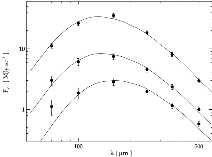
Fig. 1. Example SED fits: the datapoints are from three different positions on NGC 5457 (M 101) at R \approx 0.3, 0.5 , and 0.7 \times r_{25} , corresponding to the local average heating conditions (fitted U \approx 3, 2 and 1 , respectively, from top to bottom).
