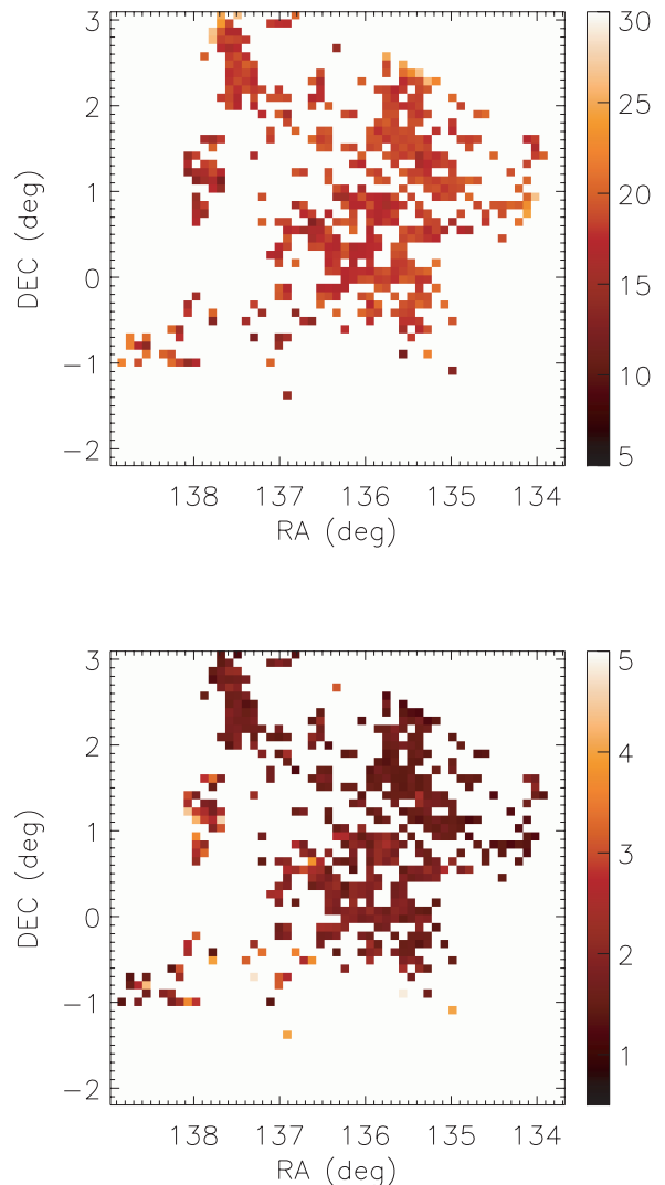
Figure 4. The dust temperature (top) and spectral emissivity parameter \beta (bottom) based on our SED fits to pixel intensities that survive the requirement that the two parameters be measured with relative uncertainty ( 1\sigma ) better than 30 per cent.
