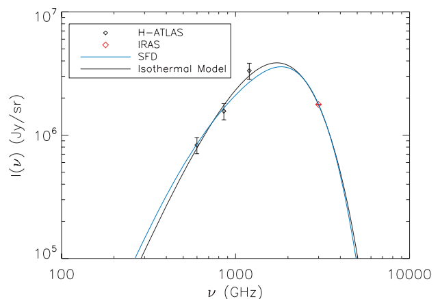
Figure 3. The Galactic dust SED averaged over the 14 \text{deg}^2 H-ATLAS SDP field and constructed by correlating SPIRE pixel intensities with 100- \mu\text{m} IRAS pixel intensity to measure the relative submm colours at each of the wavelengths (see text for details) and then scaling the IRAS mean flux over the field to SPIRE bands. The best-fitting dust temperature and spectral emissivity parameters are T_d = 19.0 \pm 2.4 K and \beta = 1.4 \pm 0.4 , respectively (black solid line). For reference, we also show the expected SED following Schlegel et al. (1998) dust map and Finkbeiner et al. (1999) frequency scaling that involves two temperature components (see Section 4.5; blue solid line).
