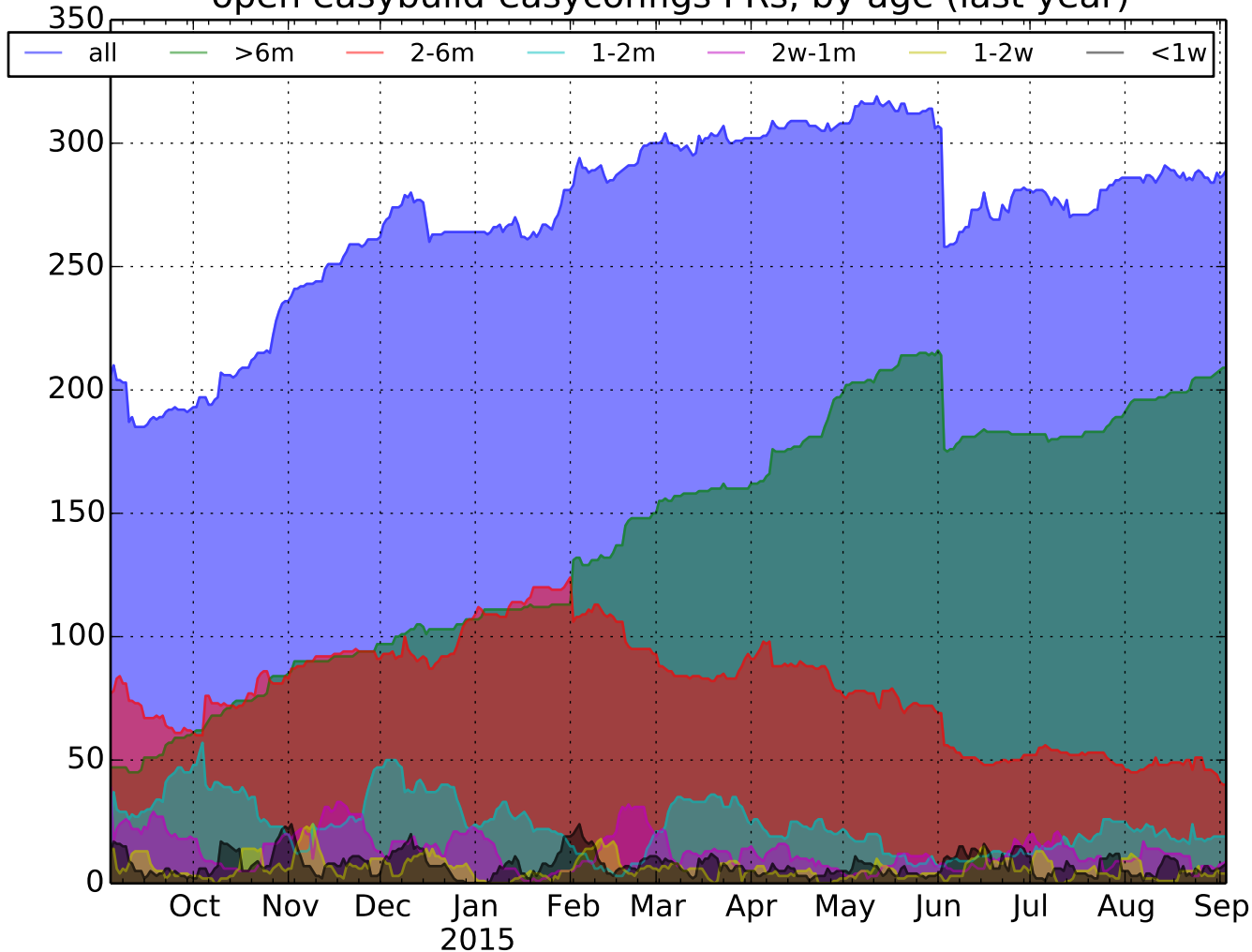
open easybuild-easyconfigs PRs, by age (last year)
