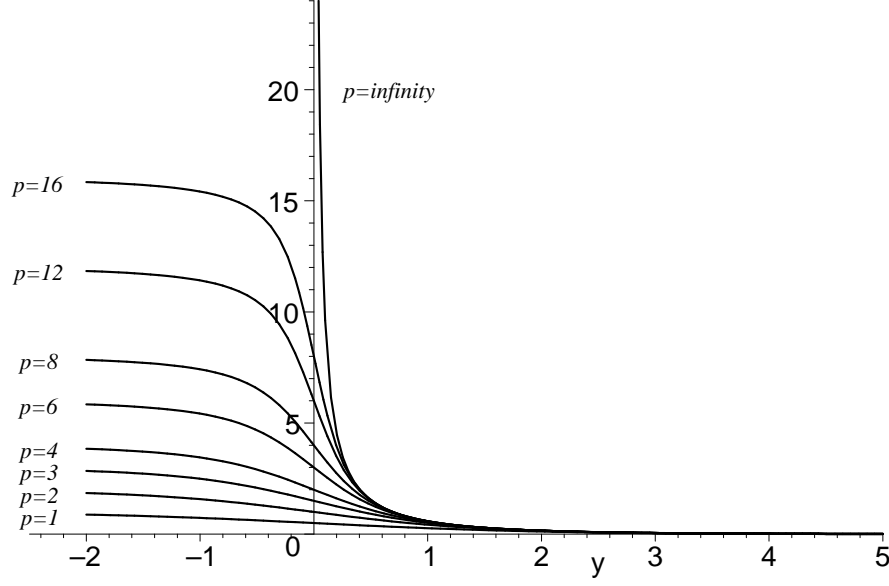
Figure 1: Graph of \bar{N}(p, 1) for p = 1, 2, 3, 4, 6, 8, 12, 16, \infty
