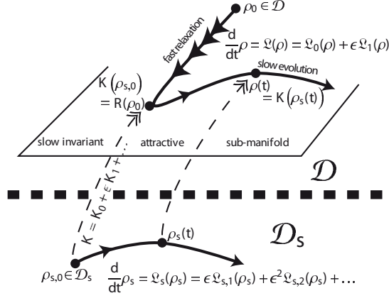
Figure 1: Adiabatic elimination, based on geometric singular perturbation theory, of the fast relaxation dynamics \frac{d}{dt}\rho = \mathfrak{V}_0(\rho) for an open-quantum system governed by the Lindbladian master equation \frac{d}{dt}\rho = \mathfrak{V}(\rho) = \mathfrak{V}_0(\rho) + \epsilon\mathfrak{V}_1(\rho) where \epsilon is a small positive parameter. It provides two asymptotic expansions of the slow dynamics. The parameterization via density operators \rho_s of the slow invariant attractive sub-manifold (related to \mathfrak{V}_0(\rho) = 0 ) is based on the map \rho = K(\rho_s) = K_0(\rho_s) + \epsilon K_1(\rho_s) + \dots . The slow dynamics corresponds to \frac{d}{dt}\rho_s = \mathfrak{V}_s(\rho_s) = \epsilon\mathfrak{V}_{s,1}(\rho_s) + \epsilon^2\mathfrak{V}_{s,2}(\rho_s) + \dots . The super-operators K_0, K_1, \dots and \mathfrak{V}_{s,1}, \mathfrak{V}_{s,2}, \dots are obtained by identifying terms of identical order versus \epsilon in the geometric invariance condition
